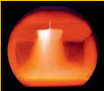
From the thermal image it is clear how strongly the air-gas mix is swirled in the glow zone combustion chamber. This constant movement significantly contributes to a low-residue combustion.
